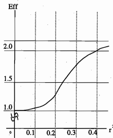
Figure 1: Relative efficiency Ratio
